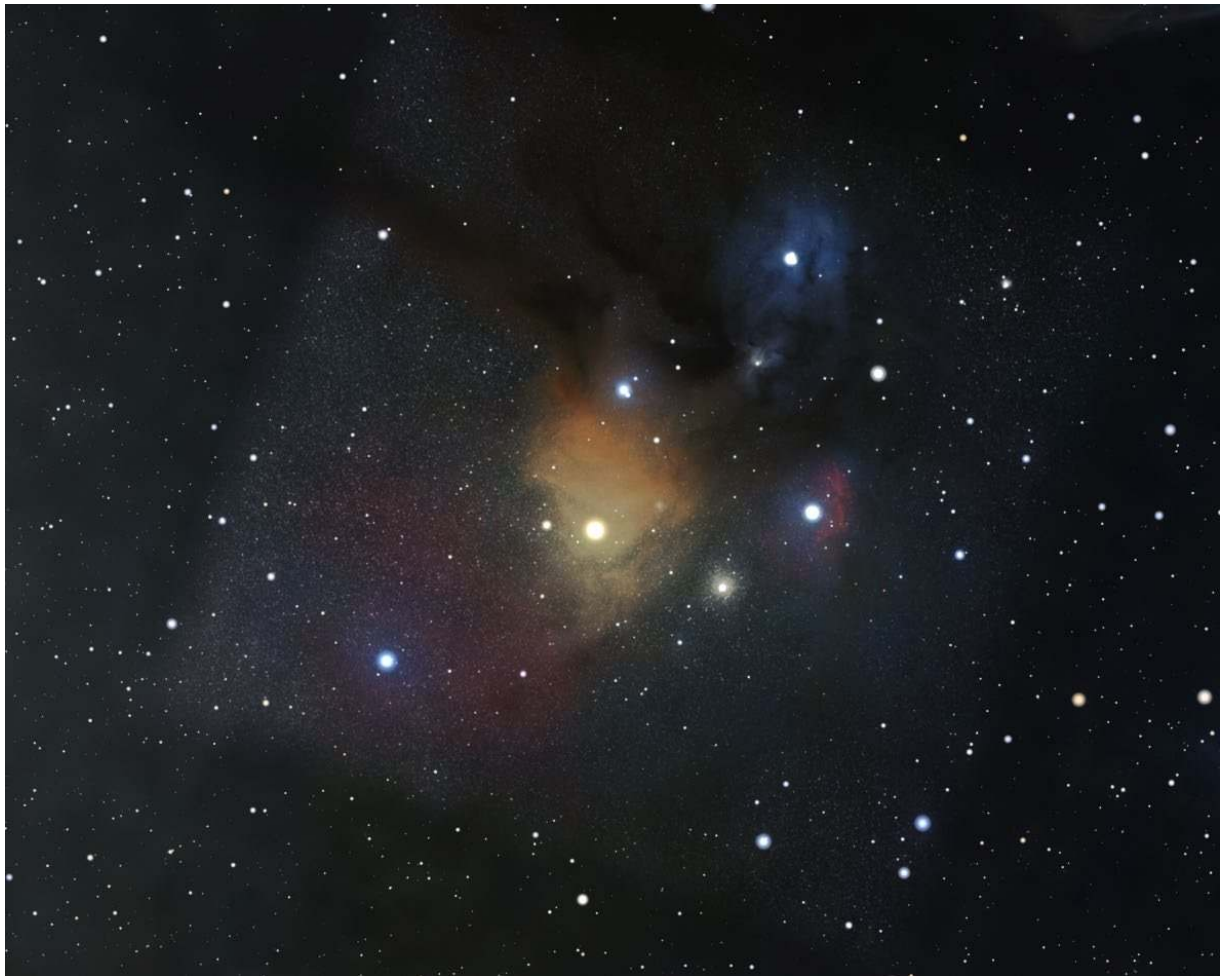
A digital map of the Rho Ophiuchi Complex. Credit: Stellarium Web
